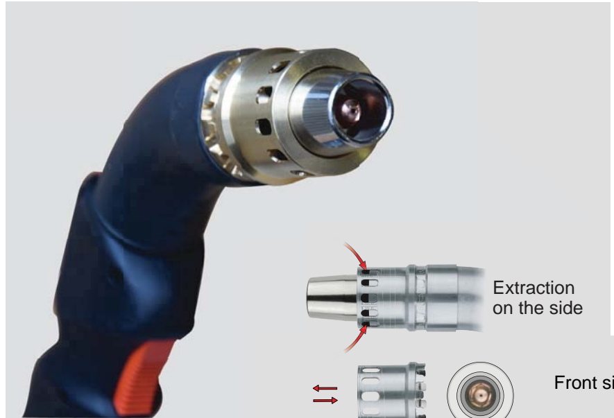
Adjustable extraction piece
